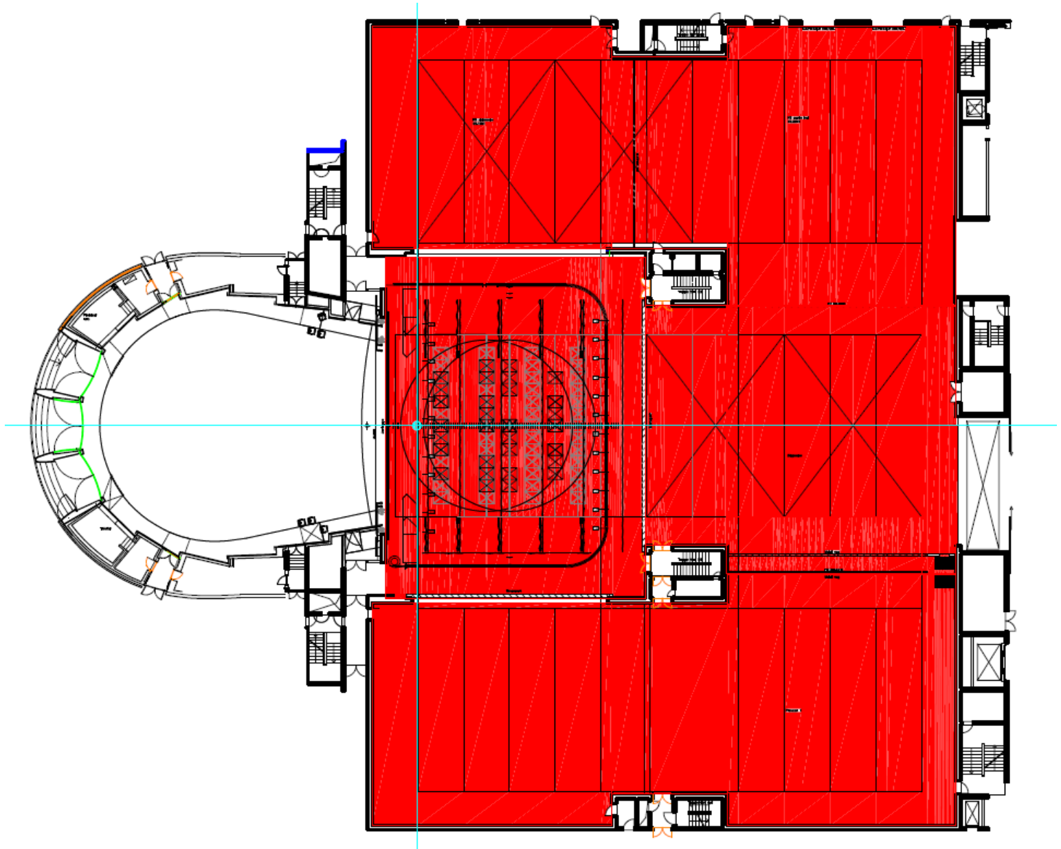
Grundriss The Royal Danish Opera, Kopenhagen
